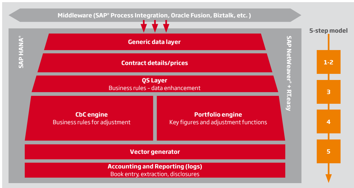
Fig. 2: IFRS15.easy architecture
